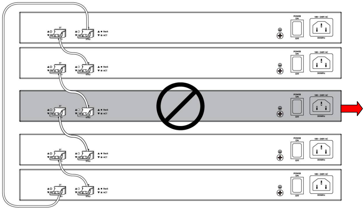
Figure 4-19-4 Remove or Replace a switch from the stack
