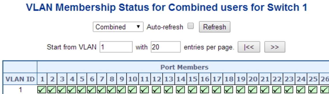
Figure 4-6-4: VLAN Membership Status for Static User page Screenshot
