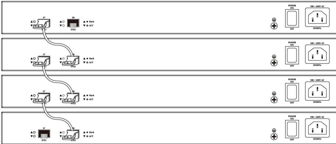
Figure 2-21 Chain Stack topology
