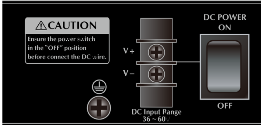
Figure 2-1-7 Rear Panel of SGS-5220-24S2XR
