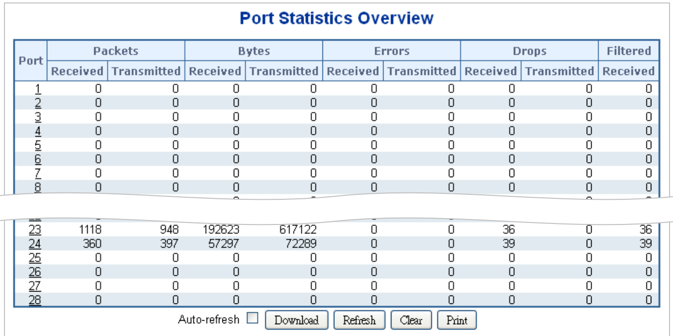
Figure 4-4-2: Port Statistics Overview page Screenshot
