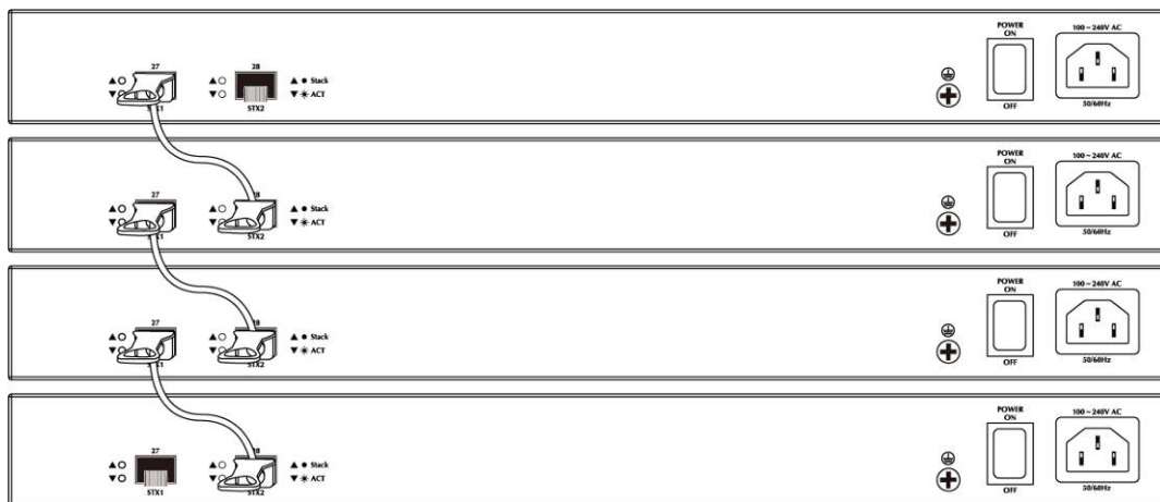
Figure 4-19-1 Chain Stack topology
