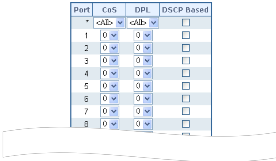
Figure 4-9-2 : QoS Ingress Port Classification page Screenshot
