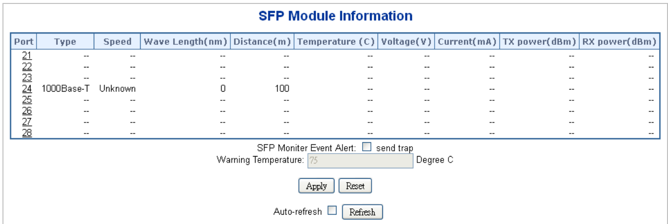
Figure 4-4-4: SFP Module Information for Switch page Screenshot
