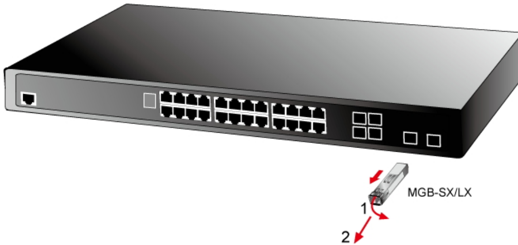
Figure 2-2-5: How to Pull Out the SFP/SFP+ Transceiver
