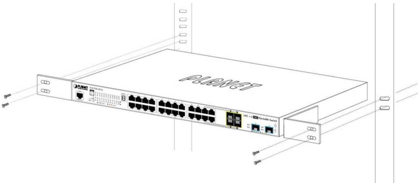
Figure 2-2-3: Mounting Managed Switch in a Rack
