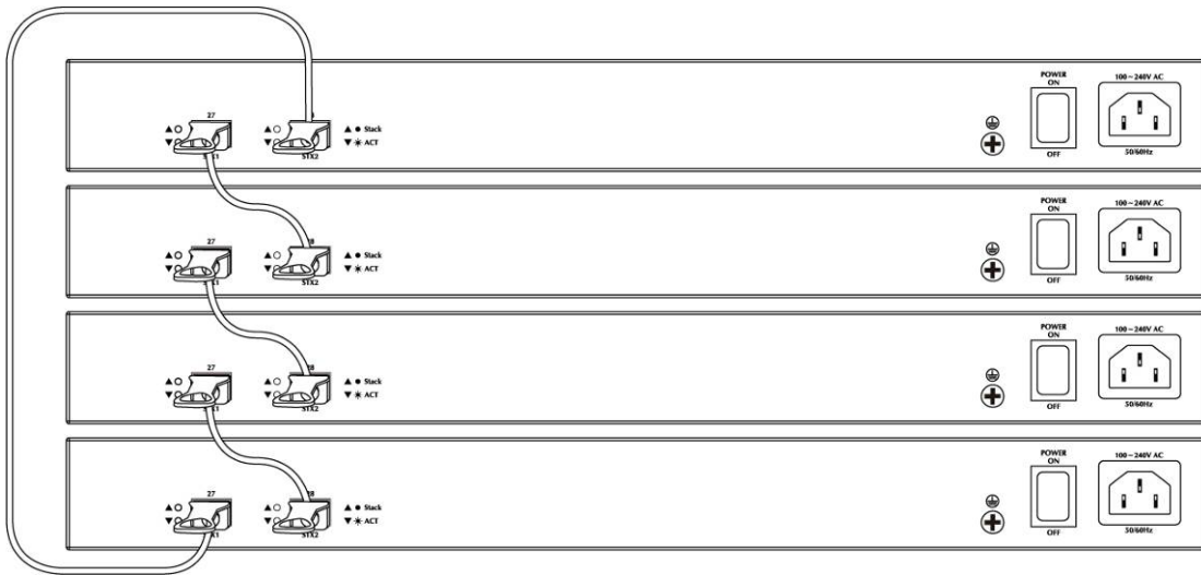
Figure 4-19-2 Ring Stack topology
