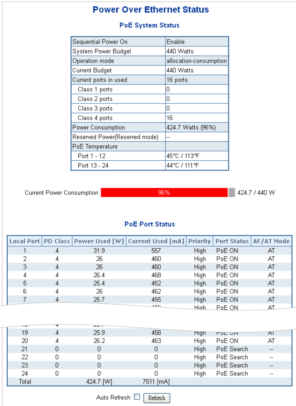
Figure 4-16-5:PoE Status Screenshot
