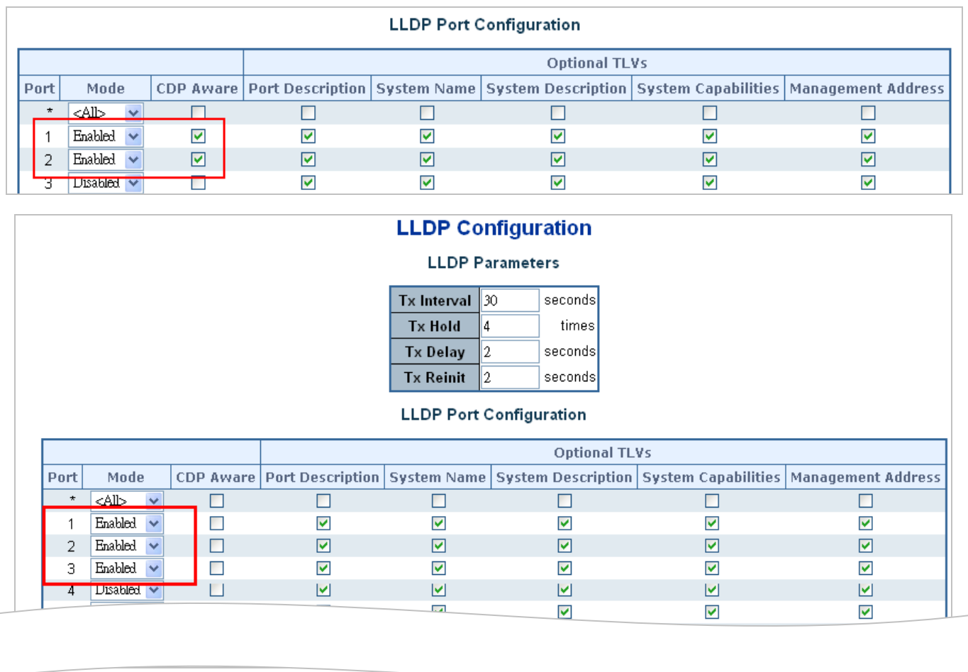
Figure 4-16-98: LLDP Configuration Screenshot
