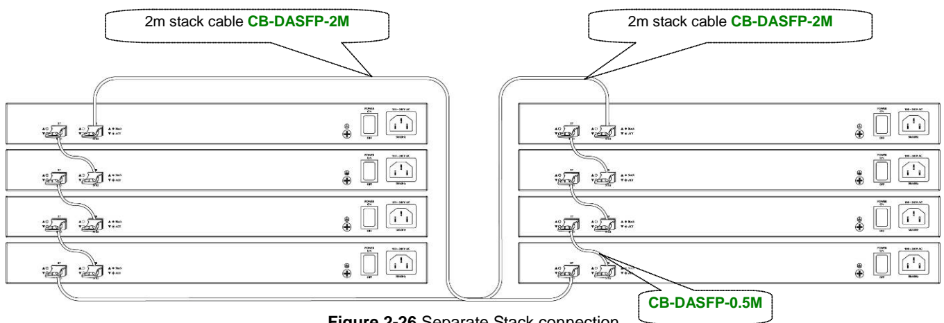
Figure 2-26 Separate Stack connection
