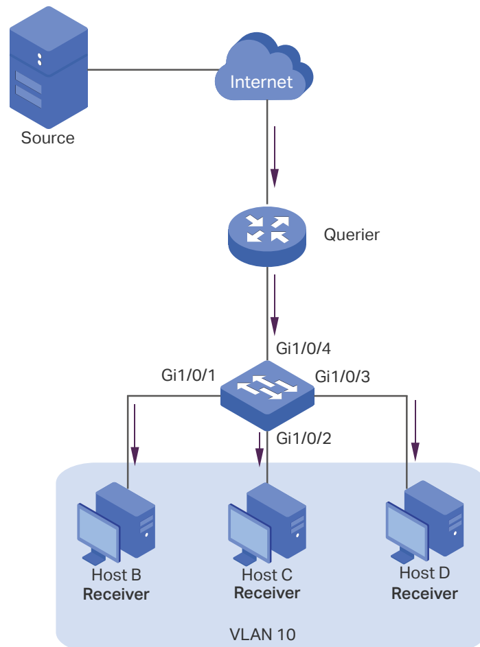
Figure 7-1 Network Topology for Basic IGMP Snooping
