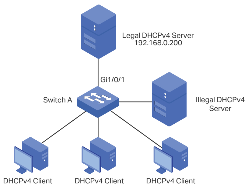
Figure 4-1 Network Topology
